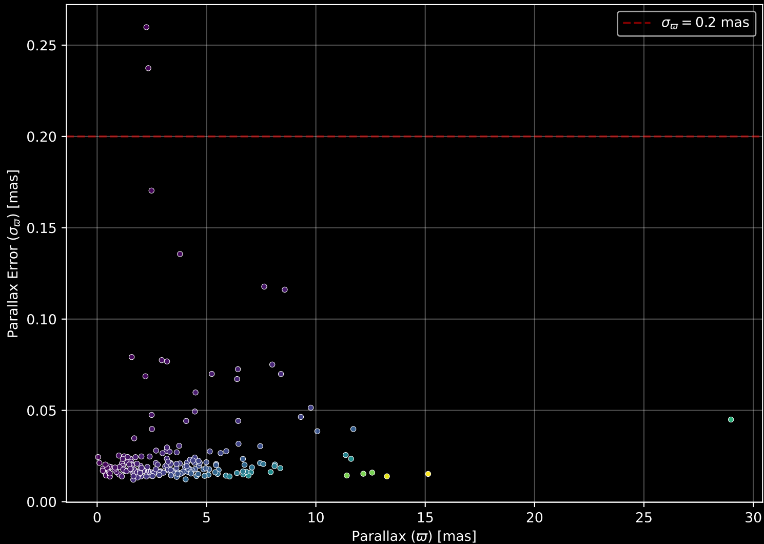
APOGEE DR17 Field: [254+58_MGA] Parallax Quality (n= 207)
