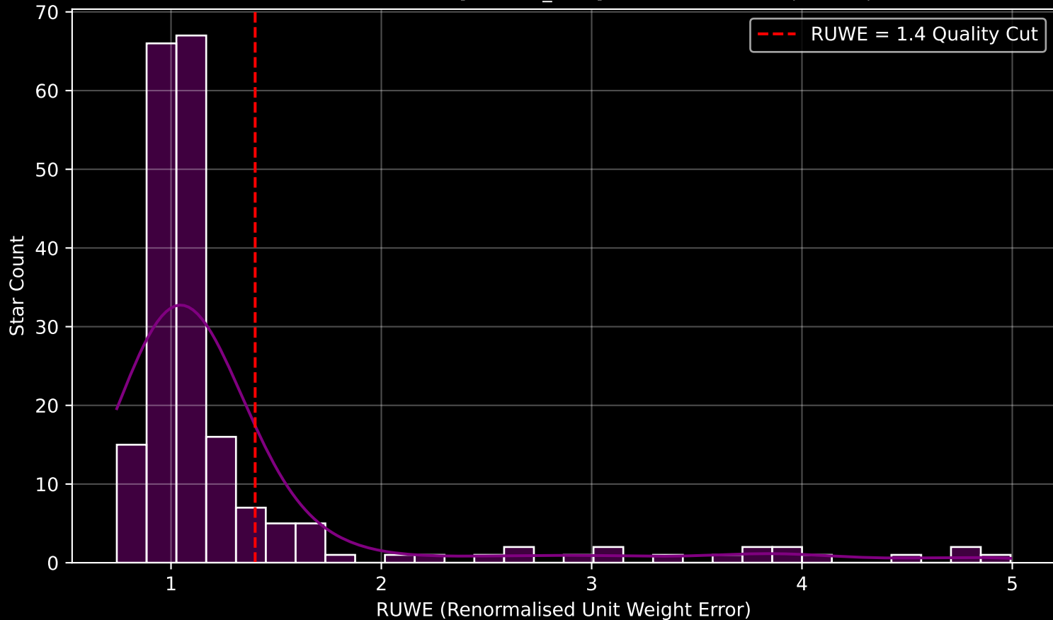
GAPOGEE DR17 Field [254+58_MGA] RUWE Distribution (n= 201)
