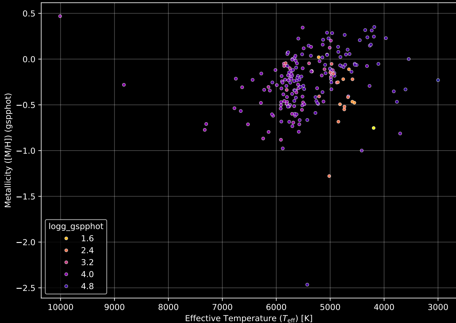
APOGEE DR17 Field: [254+58_MGA] Stellar Population Parameters (n= 207)
