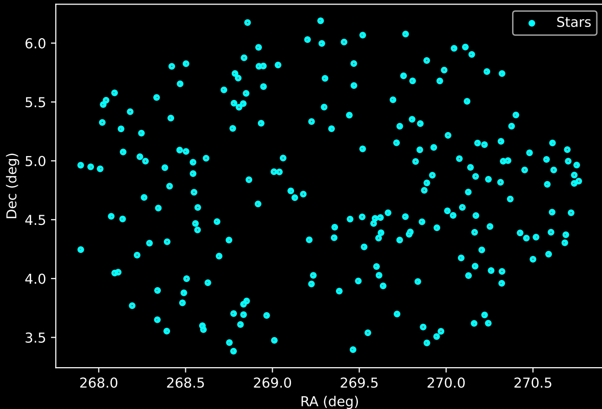
APOGEE DR17 Field: [254+58_MGA] Proper Motion Vectors for Gaia Star Field (n= 207)
