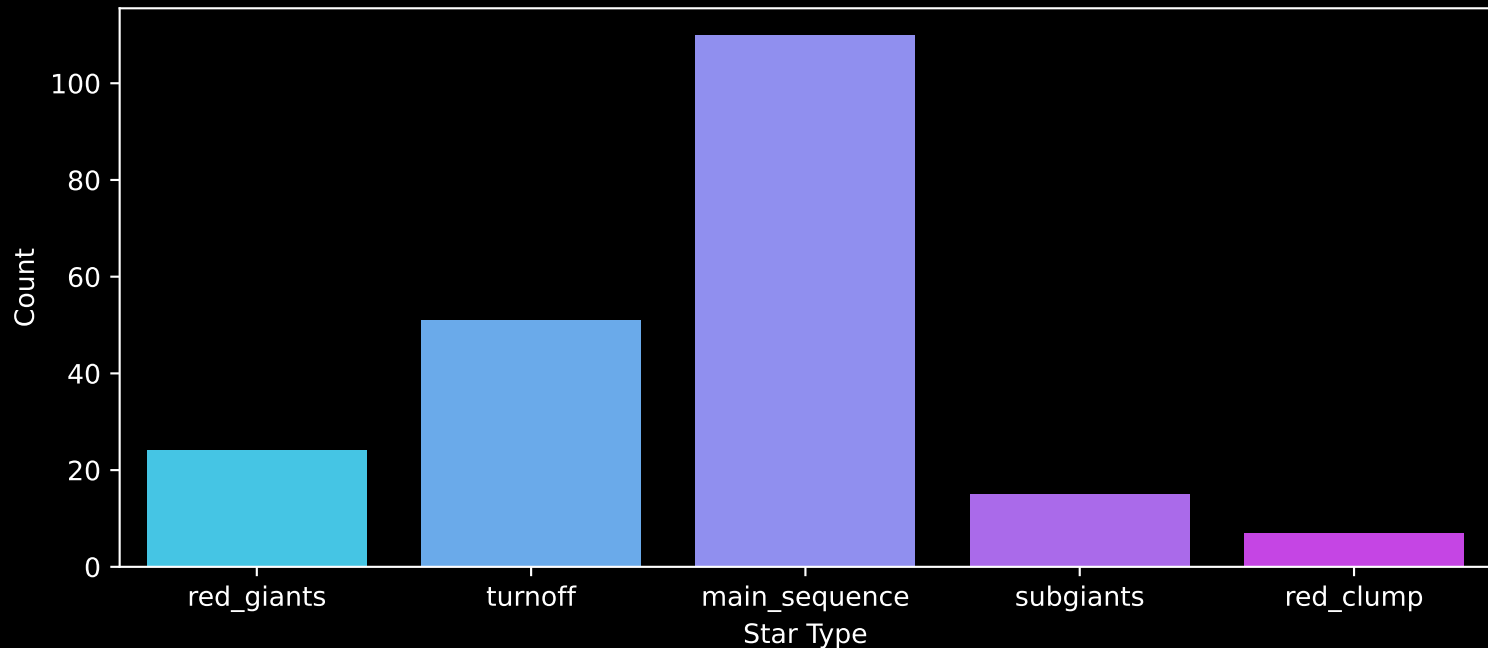
APOGEE DR17 Field: [254+58_MGA] Count plot of Star Type
