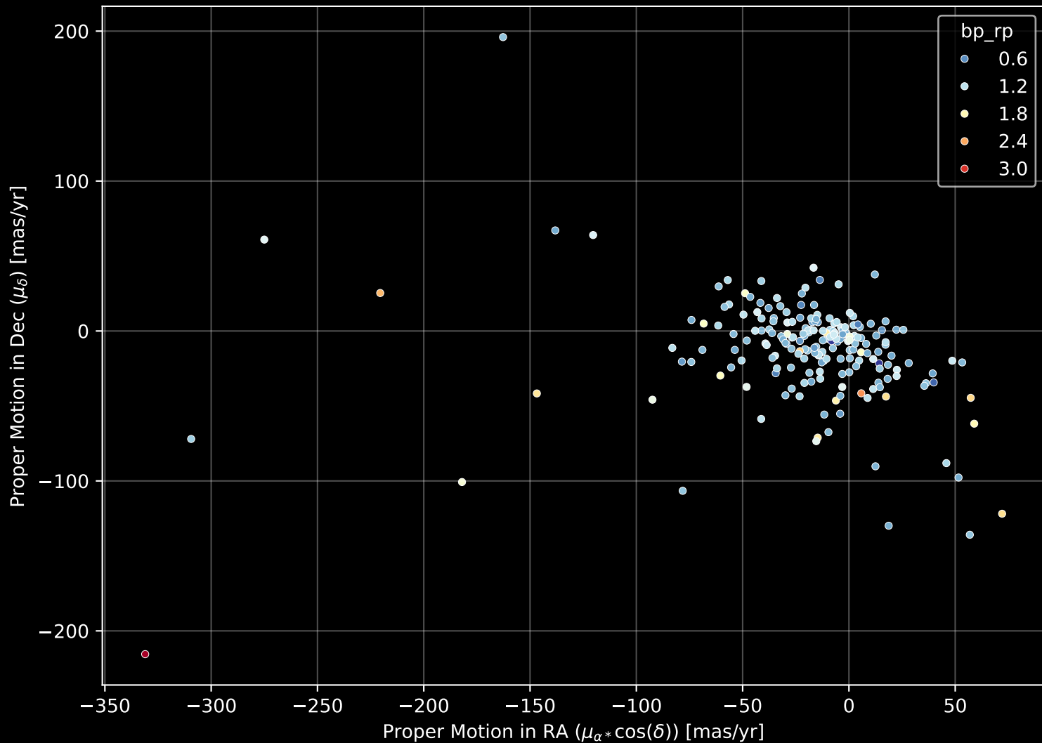
APOGEE DR17 Field: [254+58_MGA] Proper Motion Diagram (n= 207)
