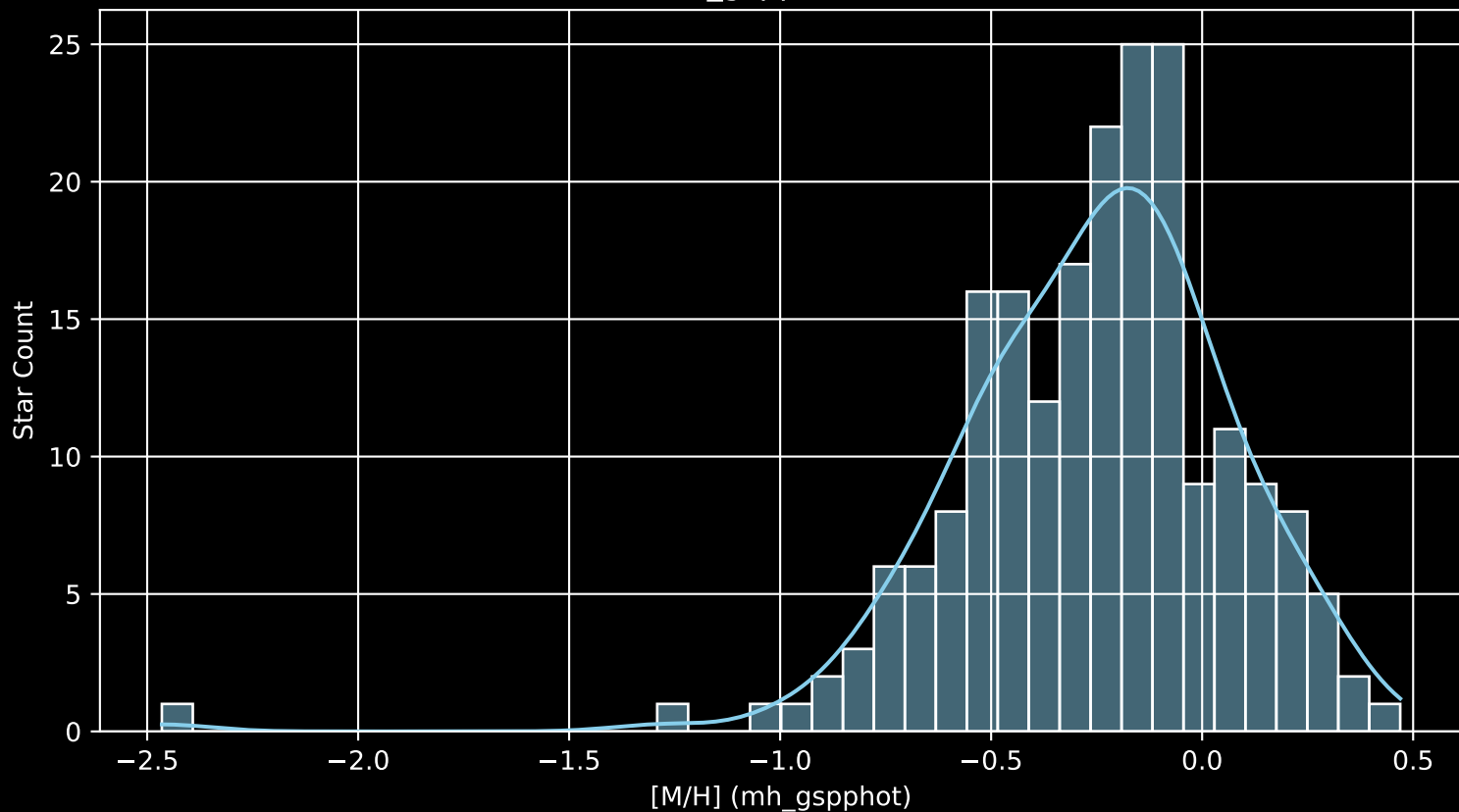
APOGEE DR17 Field: [254+58_MGA [M/H] (mh_gspphot) (n= 207)
